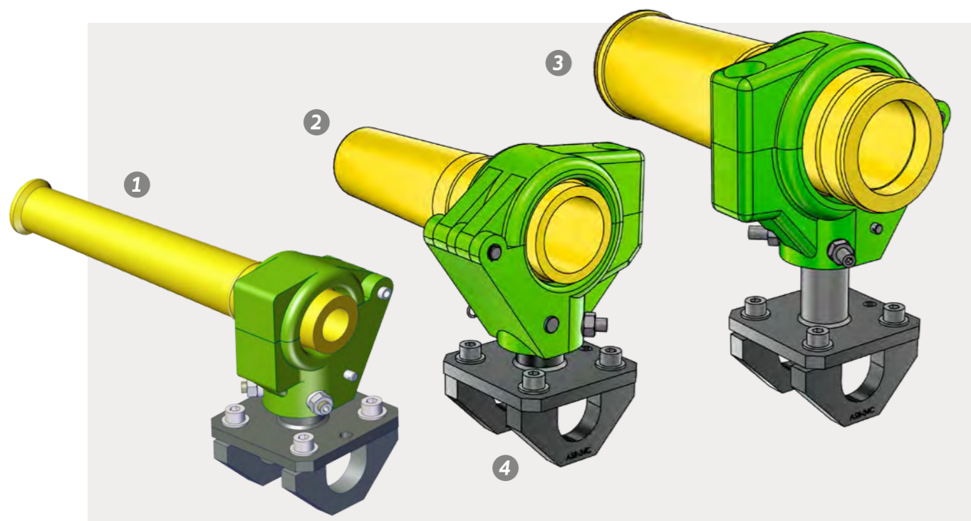
These assembly examples show yellow rotating boots, the corresponding brackets and metal supports as well as tube clamps for pipe Ø 34 mm.
