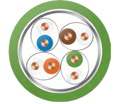
Industrial Ethernet Cat 7
