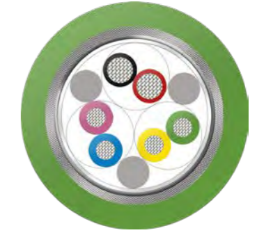
Digital feedback cable
